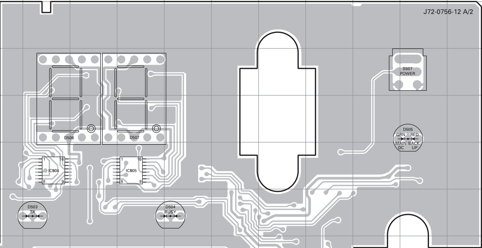
DISPLAY UNIT (X54-3330-21) Component side view (J72-0756-12)
