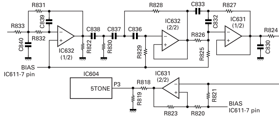
Fig. 11 5-tone decode
