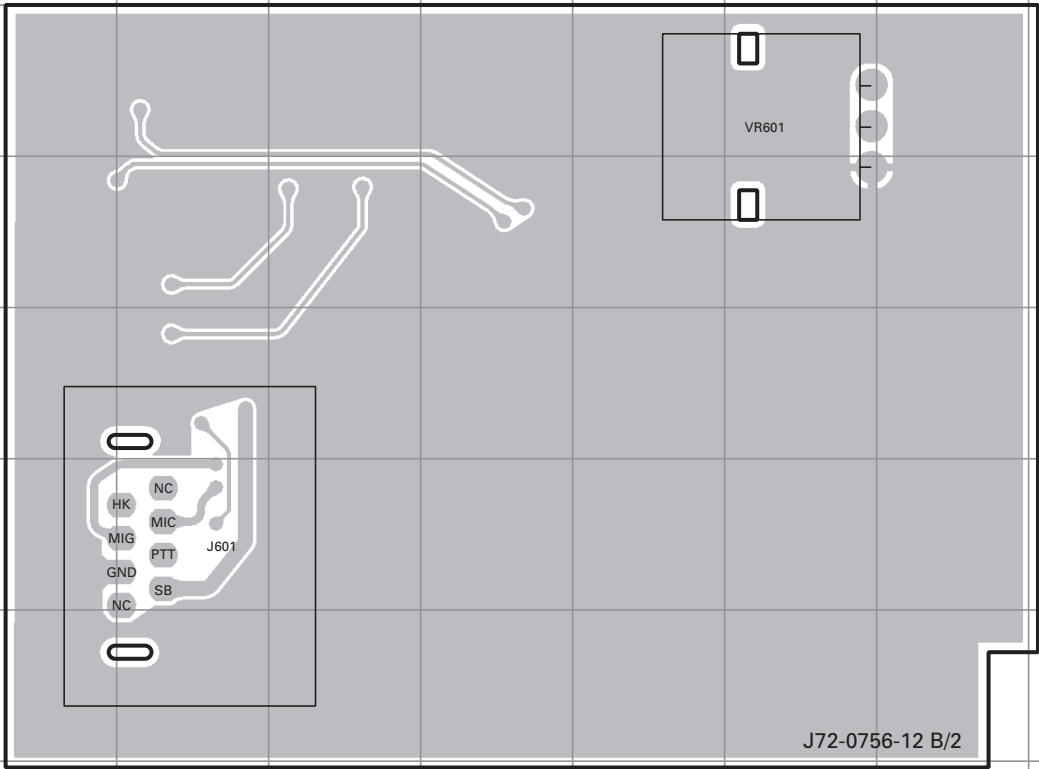
DISPLAY UNIT (X54-3330-21) Component side view (J72-0756-12)
