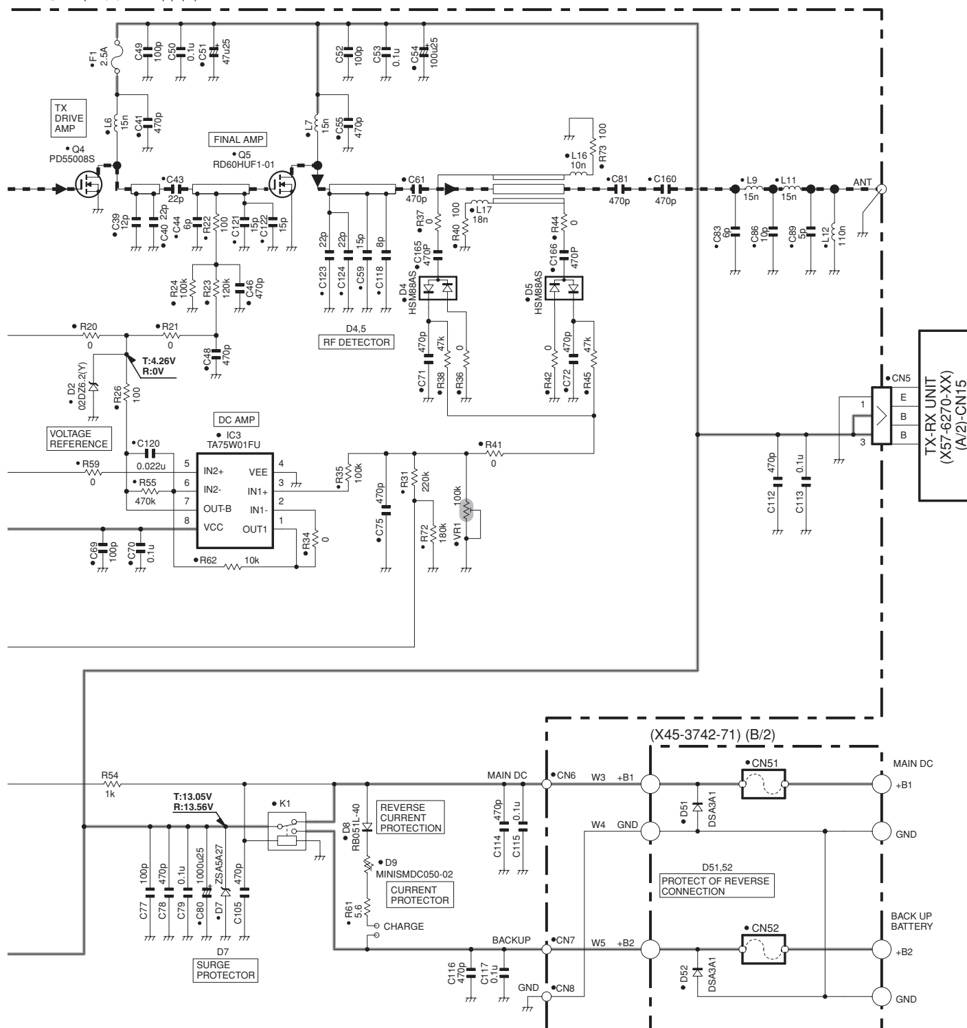
FINAL UNIT (X45-3742-71) (A/2)
